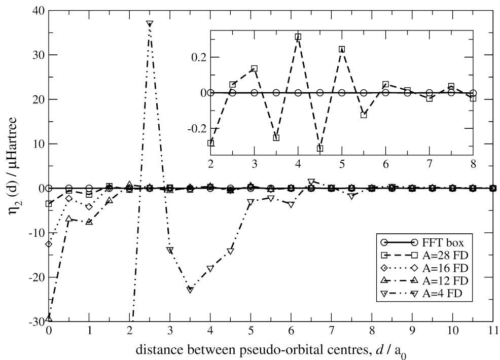
Fig. 2. Top panel: \eta_1(d) for a carbon 2s valence pseudo-orbital in a spherical support region with a radius of 6.0 a_0 . Bottom panel: \eta_2(d) for the same pseudo-orbital. The insets show a magnification of the plots for A = 28 FD and the FFT box method.
